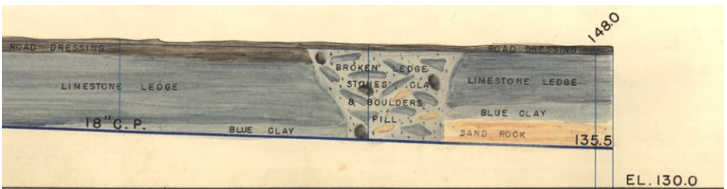
Fig. 6. The Lyndale Sinkhole likely formed along the offset between rock layers.
